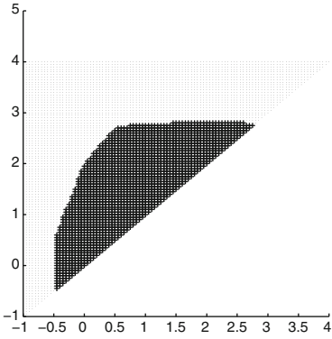
Chebyshev weight function of the second kind
