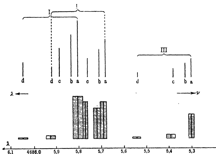
FIG. 114 a .—Spark discharge, k = 4 .
