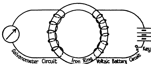
FIG. 82. Faraday's ring.
