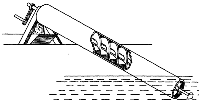
FIG. 23. Screw of Archimedes.
