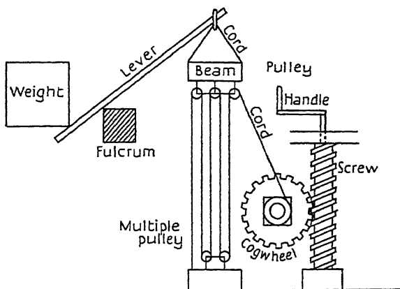
FIG. 35. Hero's mechanical repertoire.
