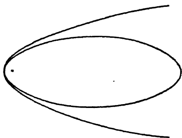
FIG. 69. Parabola and elongated ellipse, showing how they become indistinguishable from each other as they approach their common focus.
