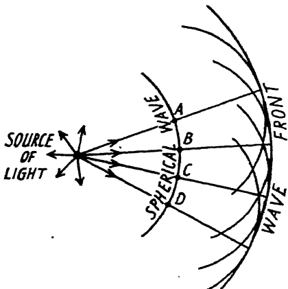
FIG. 87. Huygens's conception of 'wave-fronts'.
