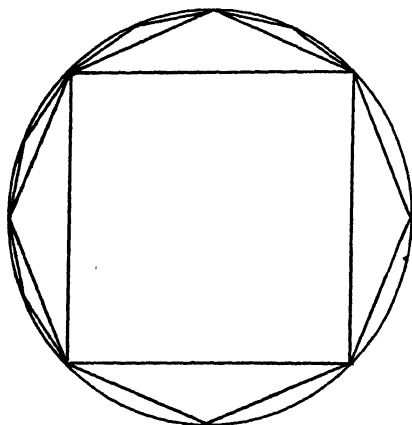
FIG. 25. Doctrine of limits.
