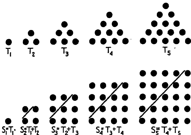
FIG. 9. Triangular and square numbers.
