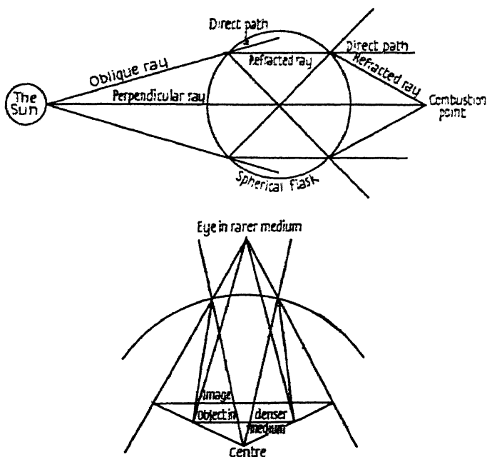
FIGS. 53 and 54. Roger Bacon's view of optical action of burning-glass and lens.
