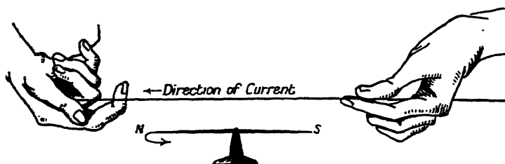
FIG. 78. Oersted's experiment on the effect of an electric current on a magnetic needle.
