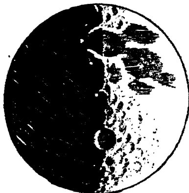
FIG. 63. The Moon as seen by Galileo in 1609.
