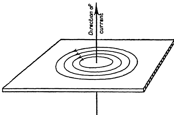
FIG. 84. Lines of force due to current in a straight conductor.
