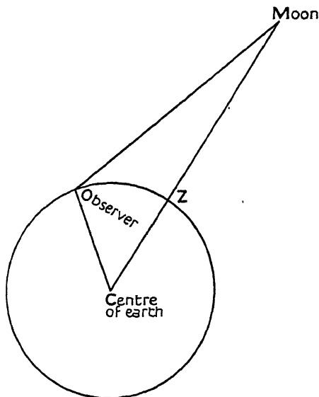
FIG. 39. Measuring Parallax of Moon.
