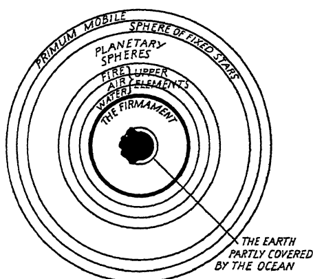
FIG. 20. The Universe of Aristotle as conceived by a medieval writer.
