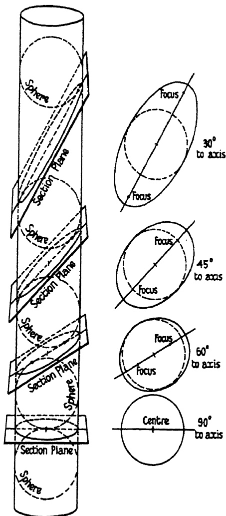
FIG. 26. The circle as special case of the ellipse, shown by series of sections through a cylinder. The cylinder of the diagram exactly contains a series of spheres; the points of contact of these with the section planes are the foci. The left figure is pictorial while the curves on the right give the true shape of the sections.
