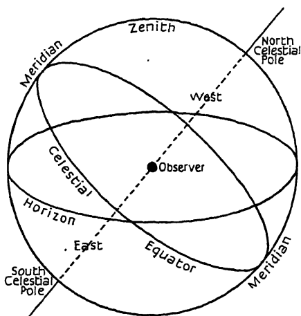
FIG. 30. The astronomical elements.
