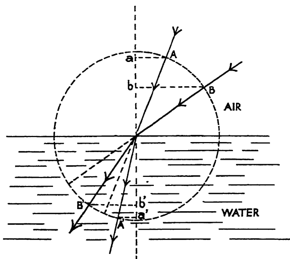
FIG. 59. Snell's law. Rays of light, passing from air into a denser medium, are bent toward the vertical to a definite amount. If AA' and BB' be two such rays \frac{A'a'}{Aa} = \frac{B'b'}{Bb} at whatever angle they strike the surface. This ratio differs for different media and the greater it is the higher is the 'refractive power' of the medium.
