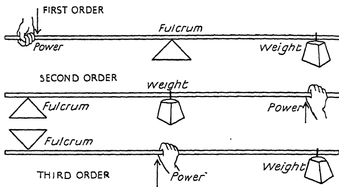
FIG. 24. The three orders of lever.
