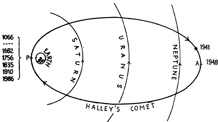
FIG. 70. Path of Halley's Comet. The position at various dates, with reference to the Perihelion, P, and Aphelion, A, is indicated.
