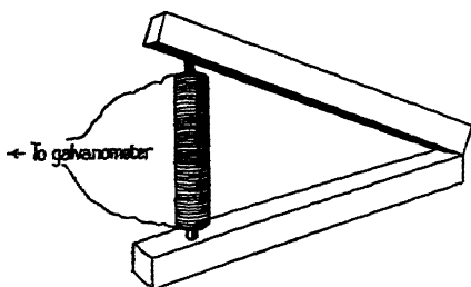
FIG. 83. Production of momentary electric current by magnetic 'make' and 'break'.
