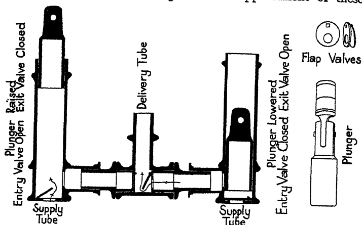
FIG. 47. Mechanism of Roman double-action pump.
