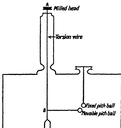
FIG. 75. Coulomb's Torsion Balance. Within a closed chamber two charged balls are insulated. One is fixed to the framework, the other attached to a wire that can be turned by a milled head. The degree of torsion needed to bring them together is a measure of the force of their mutual repulsion.
