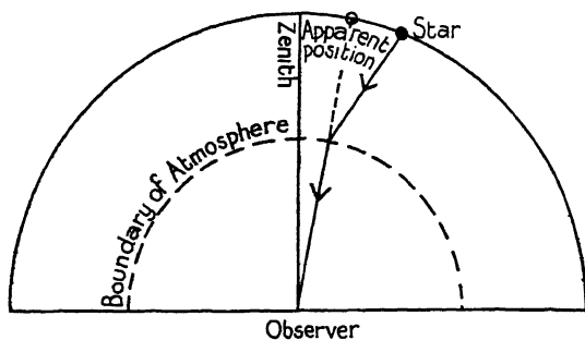
FIG. 37. Refraction of ray by atmosphere makes the apparent position of a star nearer the zenith than the real position.
