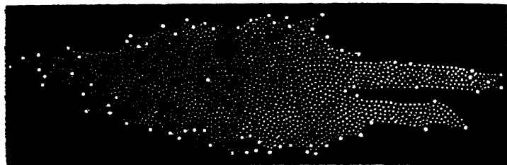
FIG. 72. Section of the Universe according to Herschel's Lens-theory.
