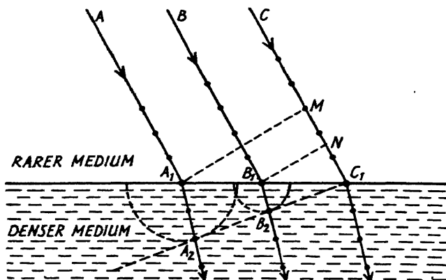
FIG. 88. Refraction in terms of Wave Theory. Beads on the lines mark equal intervals. Velocity of light in denser is two-thirds of that in the rarer medium.
