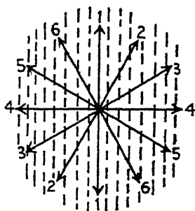
FIG. 91. Polarization of Light. The observer is supposed to view a light ray end-on as it advances toward him. The line of advance is along an axis represented by the central point. Vibrations in the ether take place in all planes through which the axis passes. These planes, from the observer's point of view, are seen as straight lines, of which six are represented. If the ray encounters a medium which acts as a grating (such as is represented by the dotted lines), permitting the passage of vibrations in only one plane (1 in diagram), the light is 'polarized'.
