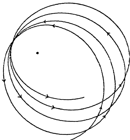
FIG. 73. Illustrating the path of a point moving in a varying ellipse.
