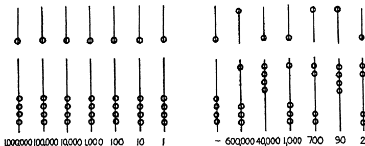
FIG. 48. Essentials of the Roman abacus, consisting of beads running on wires. On the left it is set for reckoning. On the right a total of 641,792 is represented. Without an abacal representation and in Roman figures this would need twenty-one elements, namely CCCCXXLIMVIICLXXXII.
