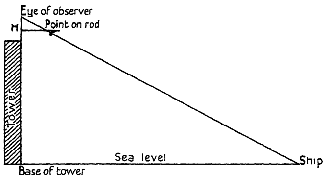
FIG. 4. Thales measures distance to ship at sea. Triangle EHP similar to triangle EBS . Therefore EH is to HP as EB is to BS . Since EH , HP , and EB are all measurable BS can be calculated.
