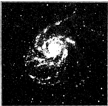
SPIRAL NEBULA
