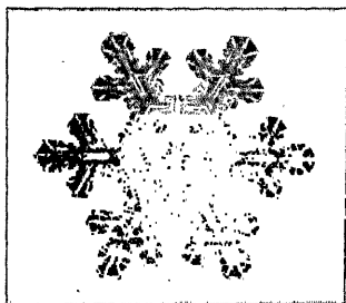
SNOW CRYSTAL
