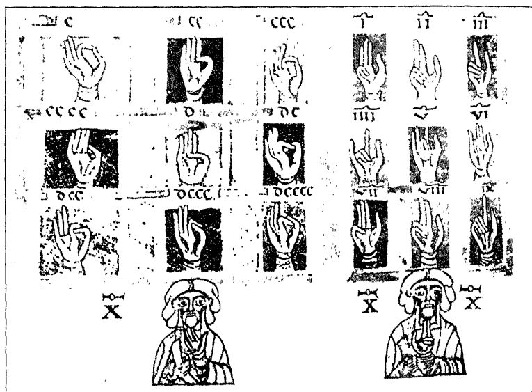
FINGER SYMBOLISM IN THE 13TH CENTURY
