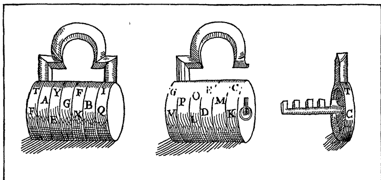
EARLY COMBINATION LOCK
