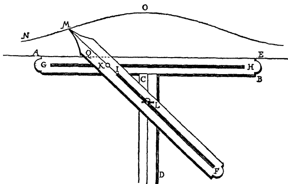
TRAMMEL FOR CONSTRUCTING THE CONCHOID
