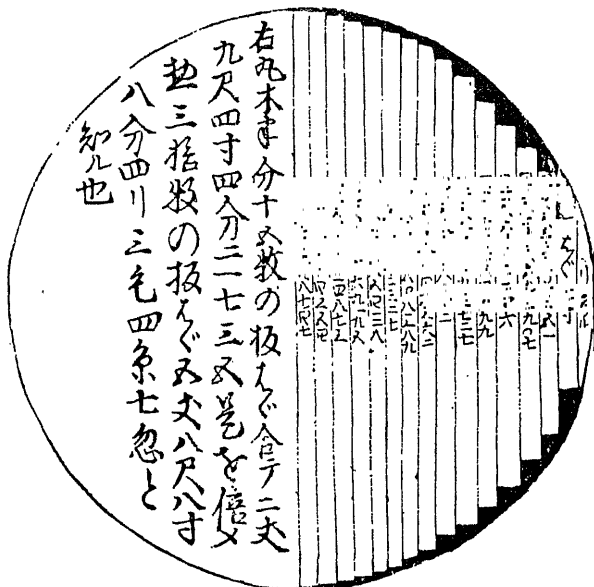
EARLY STEPS IN THE CALCULUS IN JAPAN
