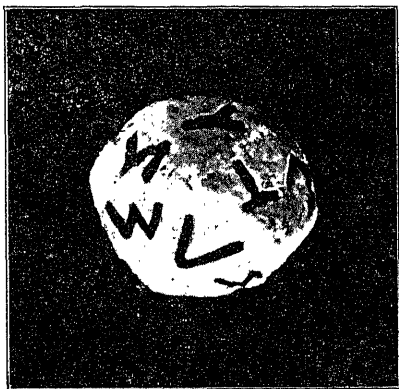
GREEK NUMERALS OF THE PTOLEMAIC PERIOD
