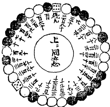
THE JOSEPHUS PROBLEM IN JAPAN
