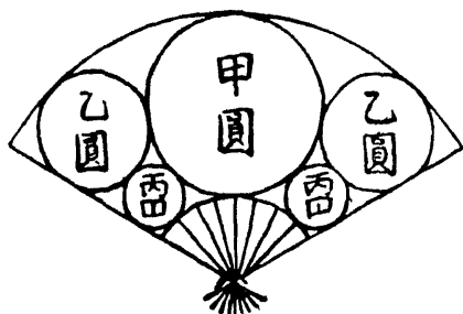
A FAN PROBLEM FROM JAPAN
