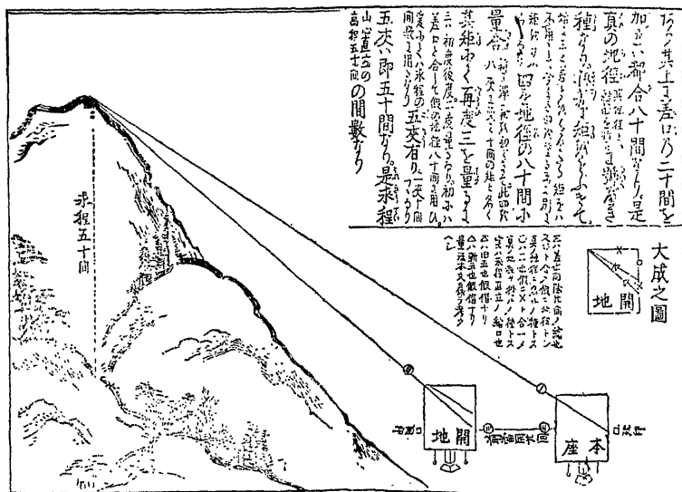
JAPANESE TRIGONOMETRY OF c. 1700
