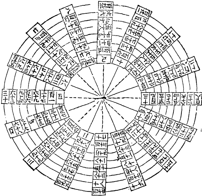
MAGIC CIRCLE OF 129 NUMBERS
