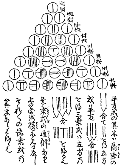
PASCAL TRIANGLE IN JAPAN
