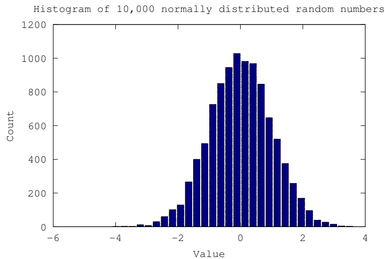
Figure 15.2: Histogram.
