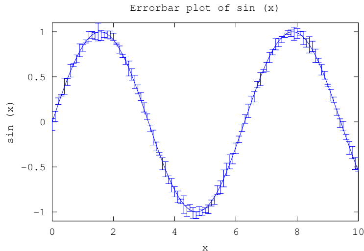
Figure 15.3: Errorbar plot.
